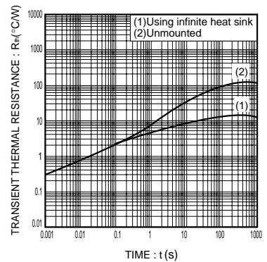
Fig.9 Transient thermal resistance
