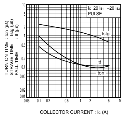
Fig.7 Switching characteristics
