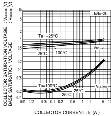
Fig.4 Collector-emitter saturation voltage - collector current Base-emitter saturation voltage
