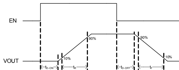
Fig.17 ON/OFF Waveform
