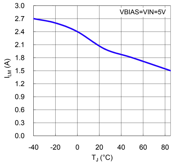
Fig.12 Current Limit vs. Temperature
