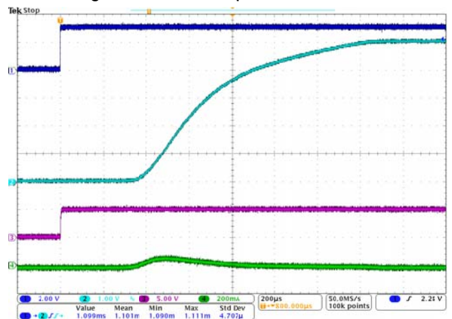
Fig.6 Turn-on Response, VIN=5.0V
