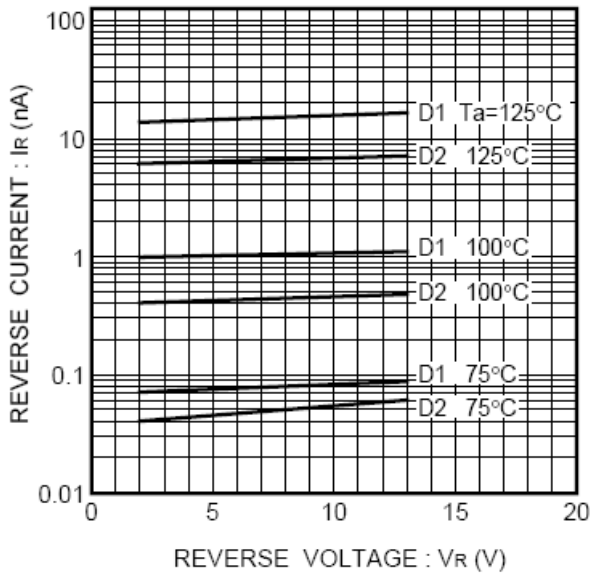
Fig.3 Reverse characteristics
