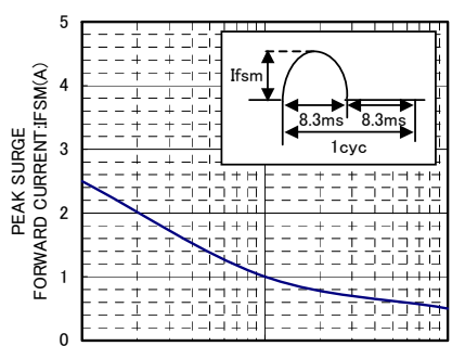
IFSM-CYCLE CHARACTERISTICS
