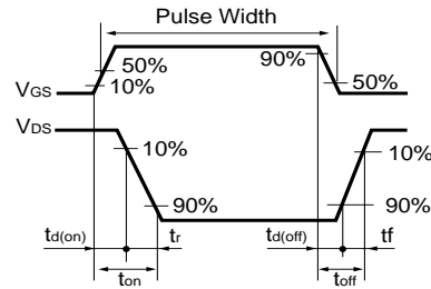
Fig.1-2 Switching Waveforms
