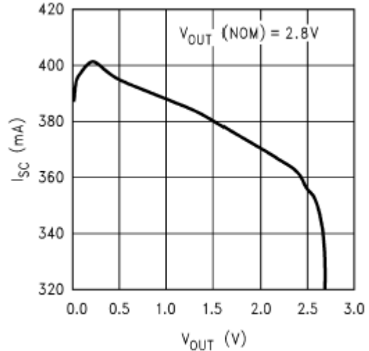
Short Circuit Current vs Output Voltage
