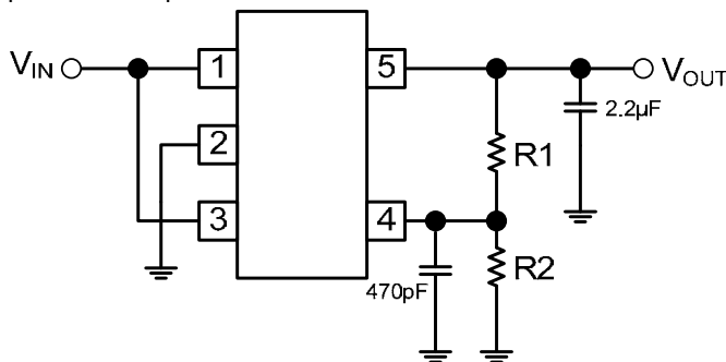
Application Circuit
