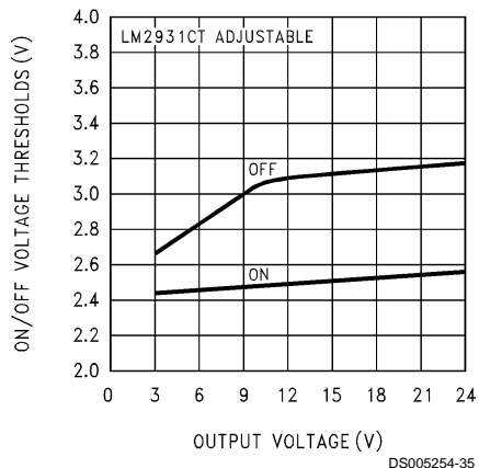
On/Off Threshold
