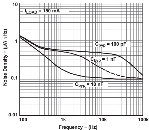
Figure 14. Output Noise Density vs Frequency
