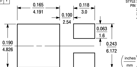
DPAK FOOTPRINT
