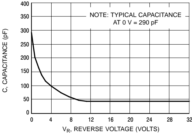
Figure 7. Typical Capacitance
