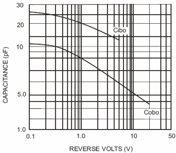
Fig. 3 Typical Capacitance
