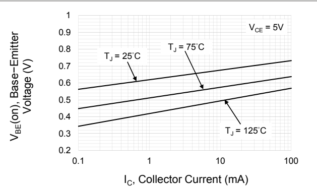
Fig.2 Base Emitter Voltage vs. Collector Current
