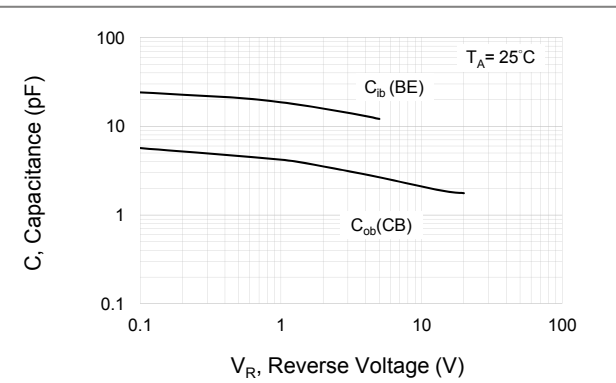
Fig.5 Typical Capacitance
