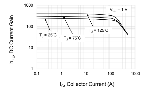
Fig.4 DC Current Gain vs. Collector Current
