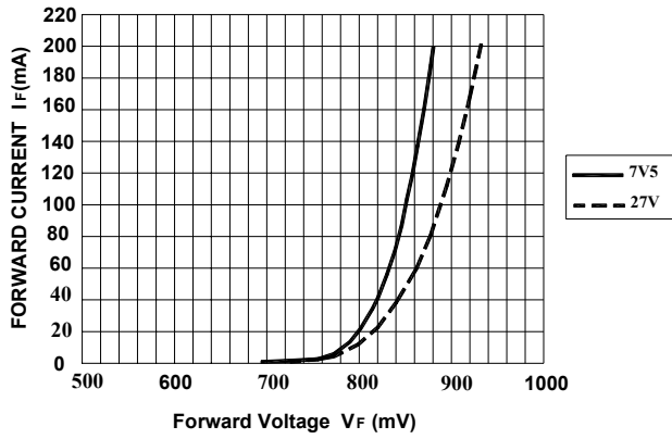
Typical Forward Voltage
