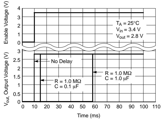
Figure 33. Delayed Turn-on
