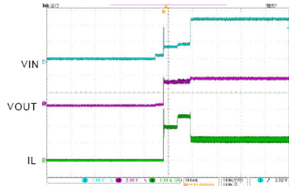
6. Start-Up Waveform
