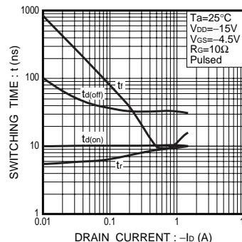
Fig.9 Switching Characteristics
