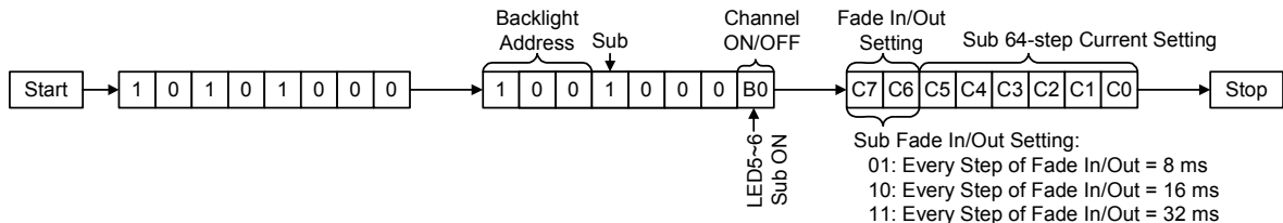
Figure 2. Control Sequences of LDO Setting and LEDDimming
