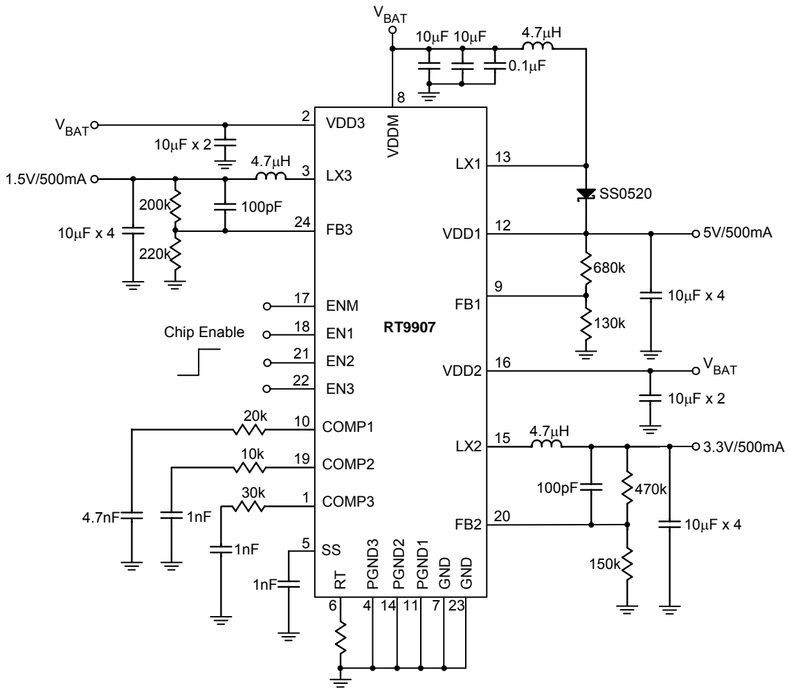
Figure 1. Typical Application Circuit for 1-cell Li+ Battery
