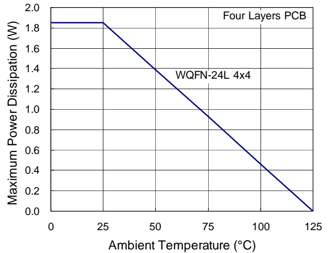
Figure 2. Derating Curves for RT9912A Packages
