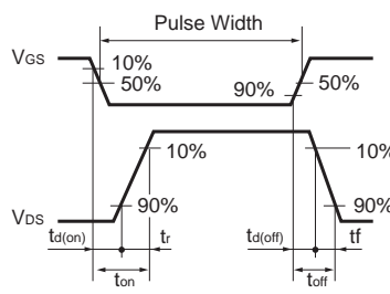
Fig.1-2 Switching Waveforms
