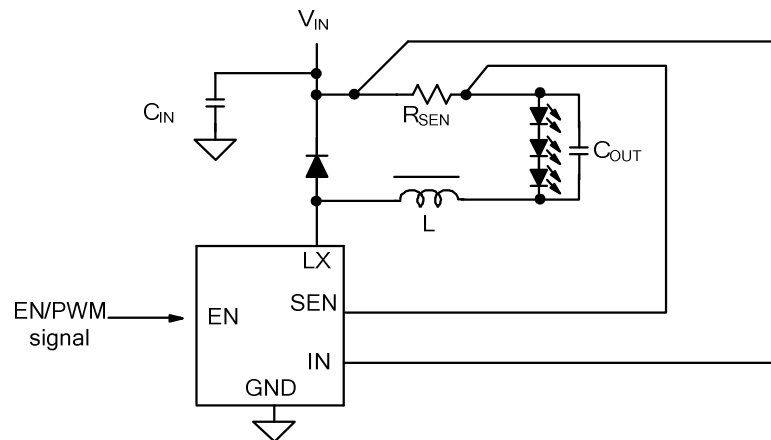
Figure 1. Schematic diagram
