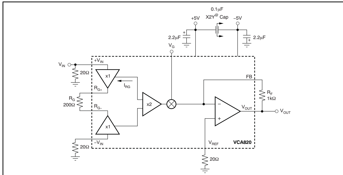
Figure 76. DC-Coupled, A_{V_{MAX}} = 20\text{dB} , Bipolar Supply Specification and Test Circuit
