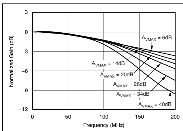
Figure 85. SO-14 Recommended R_F and R_G versus A_{VMAX}
