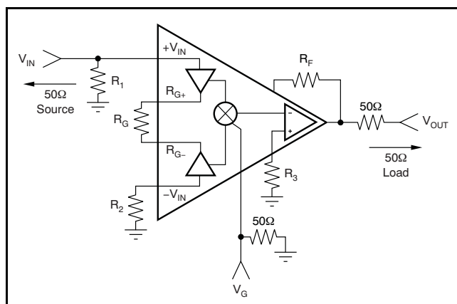
Figure 84. Test Circuit
