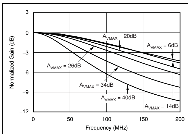
Figure 86. MSOP-10 Recommended R_F and R_G versus A_{VMAX}
